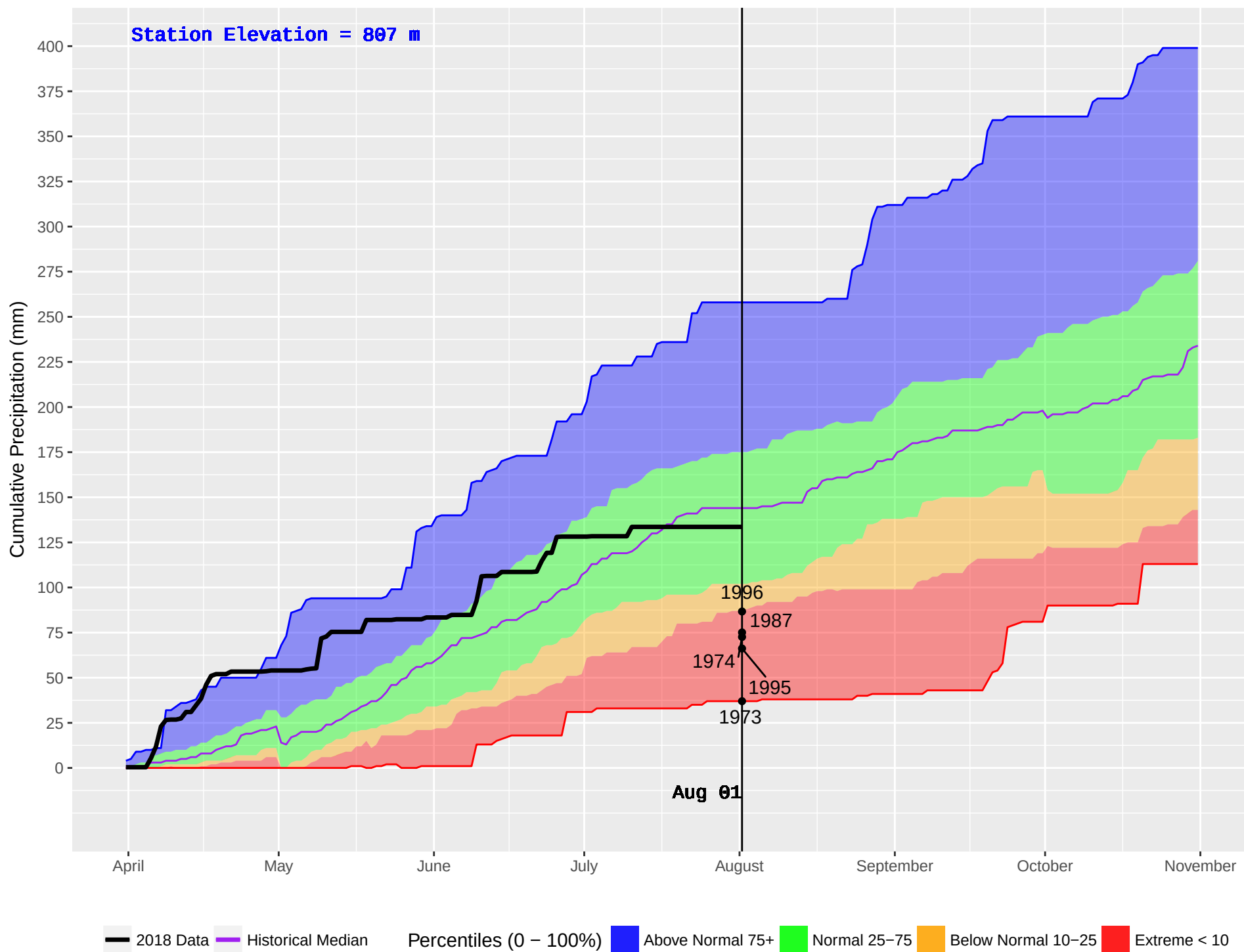
BEAVERDELL (390) : Historical (1970–2016) and Current (2018) Daily Cumulative Precipitation
