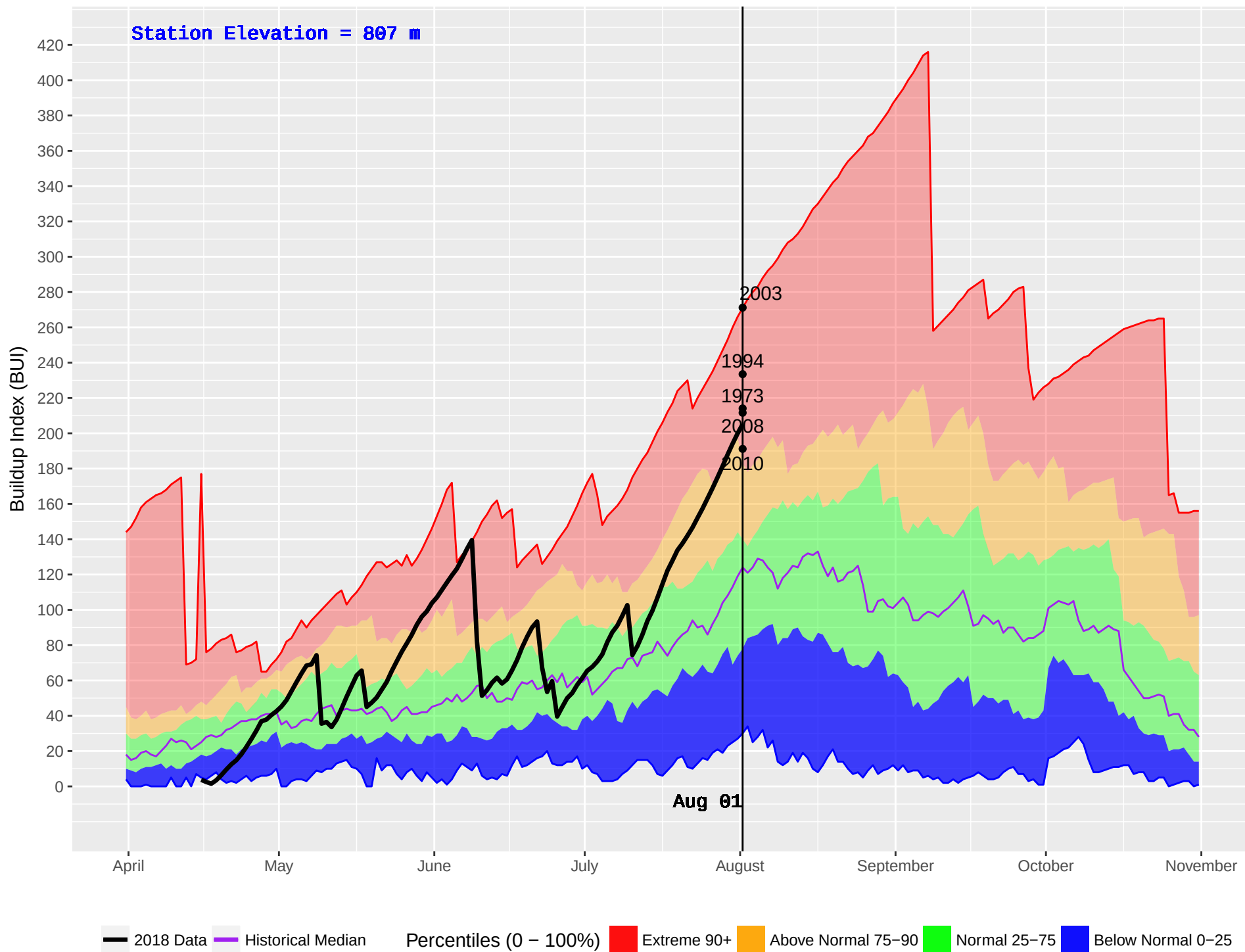
BEAVERDELL (390) : Historical (1970–2016) and Current (2018) Daily Buildup Index (BUI)
