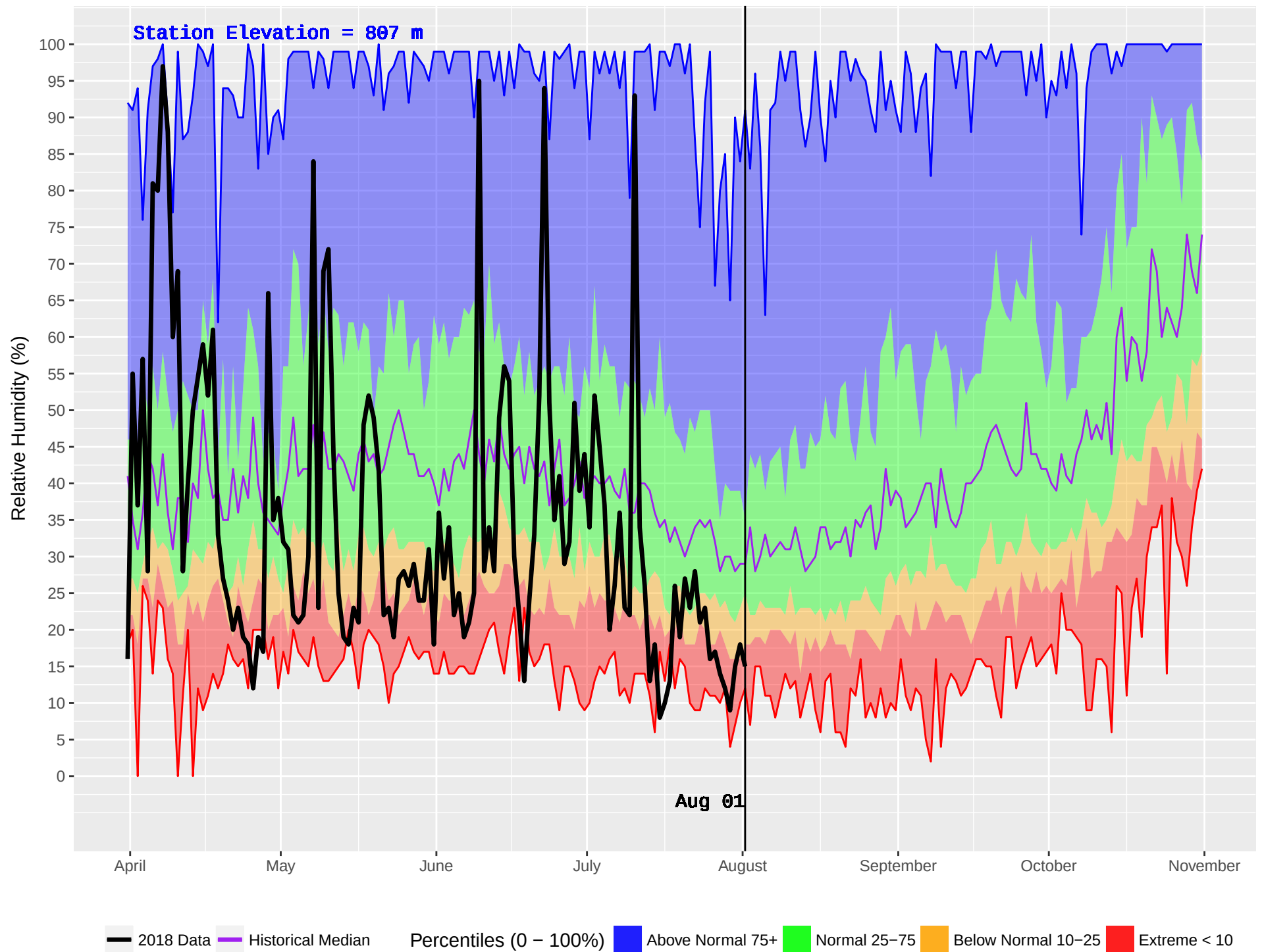
BEAVERDELL (390) : Historical (1970–2016) and Current (2018) Daily Relative Humidity
