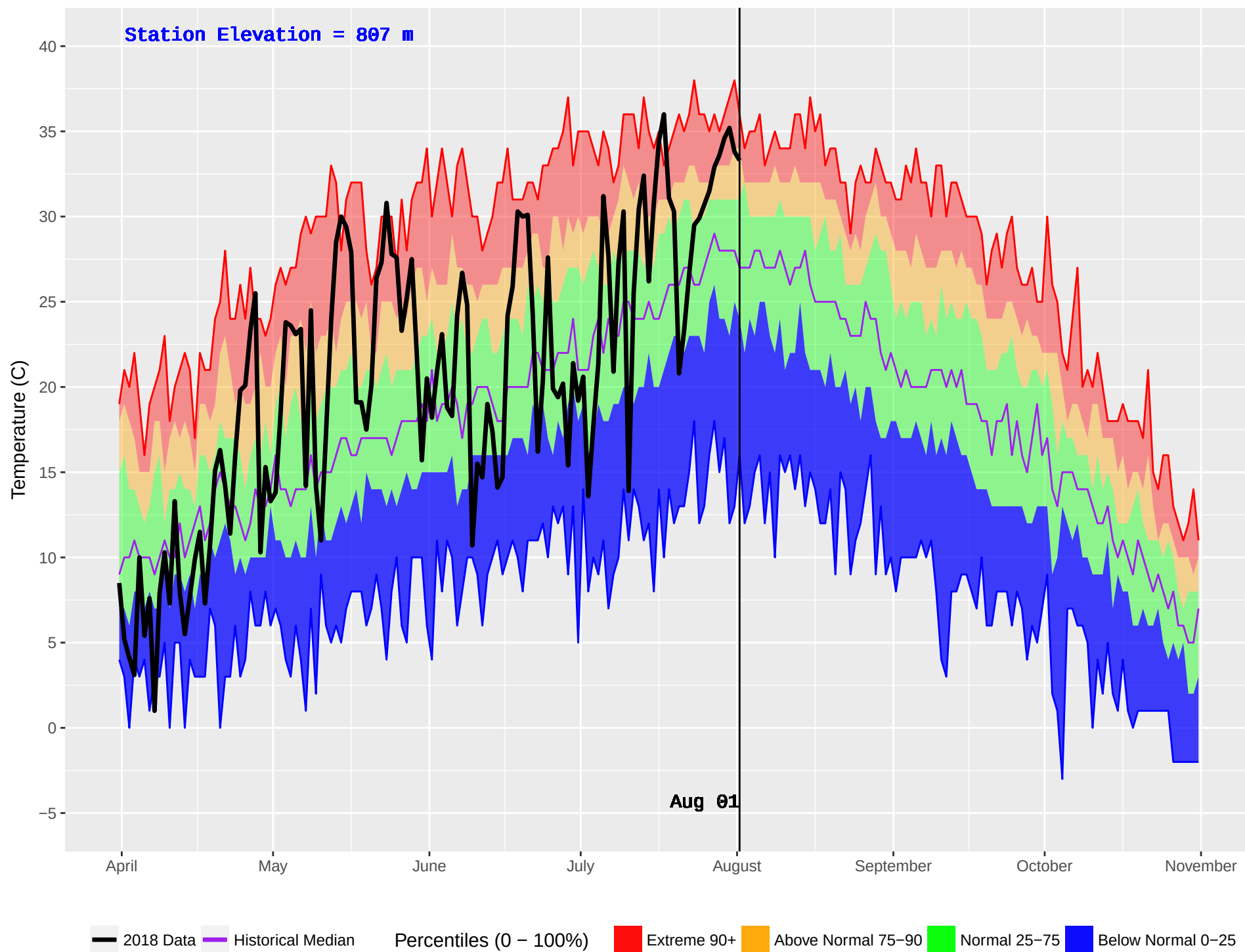
BEAVERDELL (390) : Historical (1970–2016) and Current (2018) Daily Temperature
