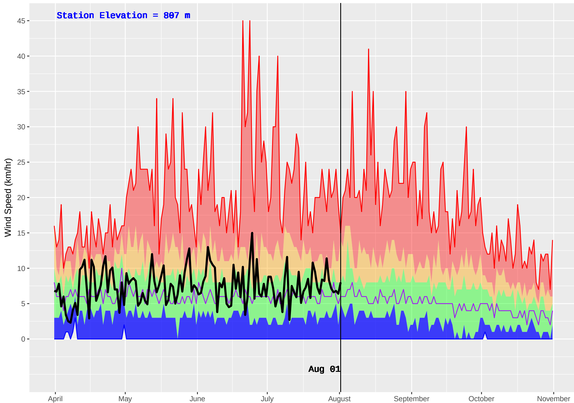
BEAVERDELL (390) : Historical (1970–2016) and Current (2018) Daily Wind Speed
