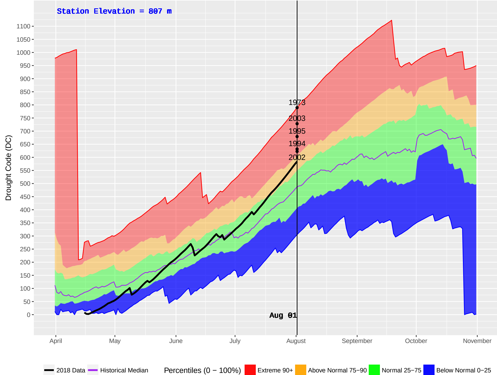
BEAVERDELL (390) : Historical (1970–2016) and Current (2018) Daily Drought Code (DC)
