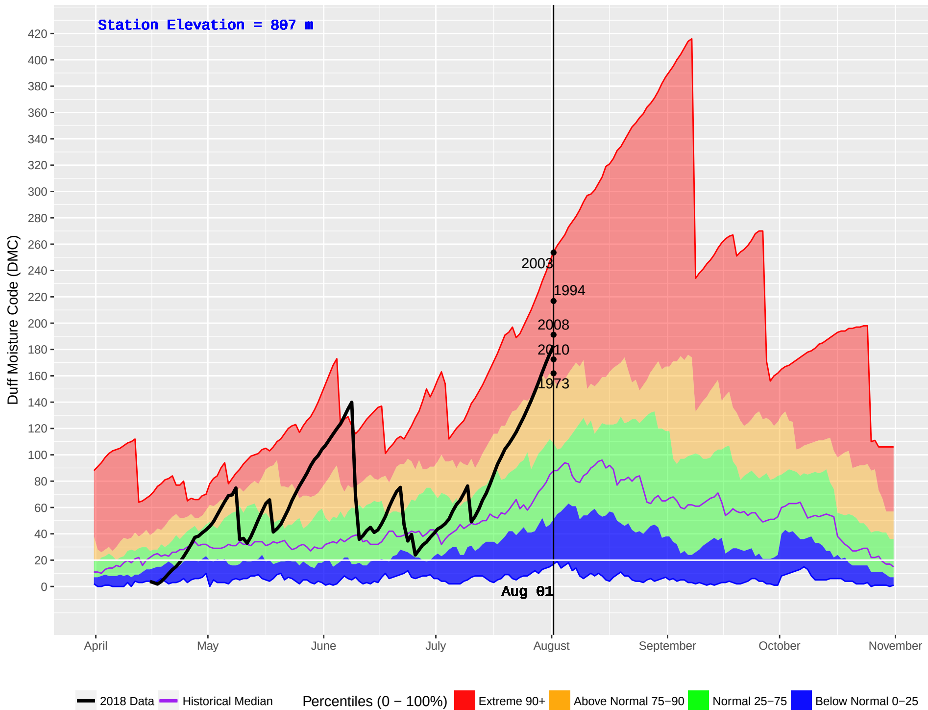
BEAVERDELL (390) : Historical (1970–2016) and Current (2018) Daily Duff Moisture Code (DMC)
