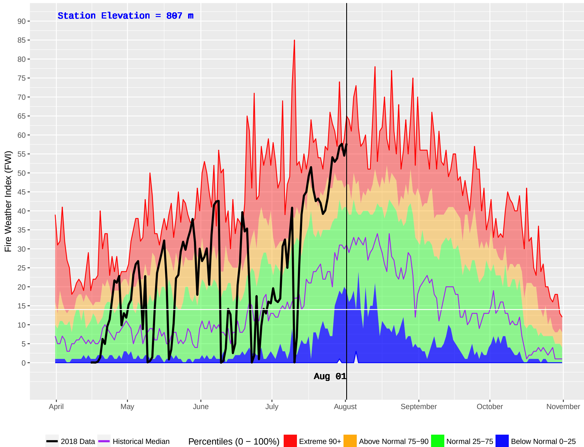
BEAVERDELL (390) : Historical (1970–2016) and Current (2018) Daily Fire Weather Index (FWI)
